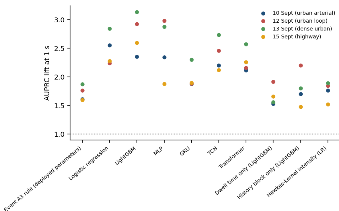
Figure 5.4 One-second AUPRC lift by learner, with each held-out campaign drawn separately. The spread across campaigns is wider than the spread across learners.
