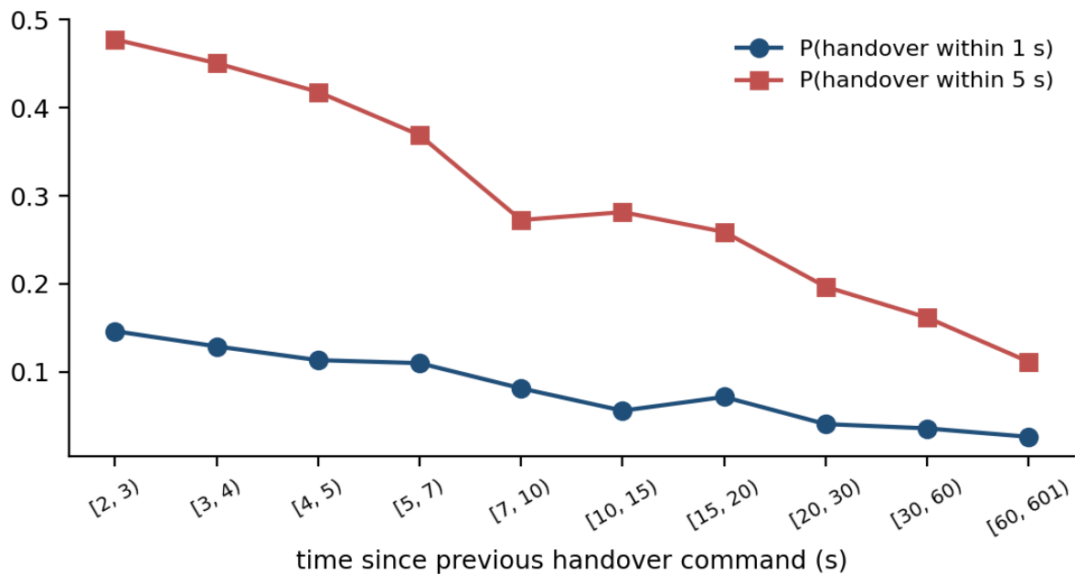
Figure 5.13 Probability of a handover command within one and five seconds against the time since the previous command, computed from signalling timestamps.
