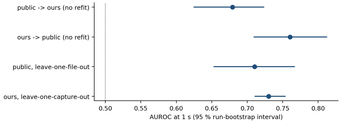
Figure 5.11 Transfer to an independently collected dataset on the same network, with both domains built from L3 signalling alone. Bars are 95 % bootstrap intervals over runs.
