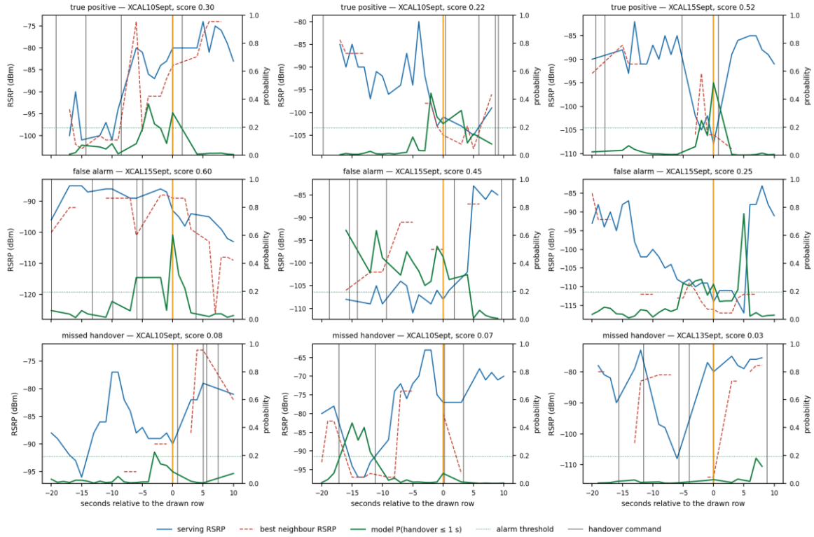
Figure 5.20 Nine cases drawn uniformly at random, with a fixed seed, from the out-of-fold predictions at the 5 % false-positive operating point. Blue is the serving cell's RSRP, red the best neighbour's, green the model's probability of a command within one second against the right axis, the dotted line the alarm threshold, black lines are handover commands and the orange line is the drawn row. Nothing here was selected for being illustrative.
